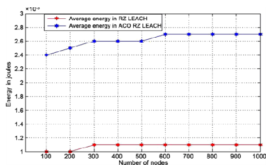
Figure 2. Average remaining energy evaluation in existing RZ LEACH & proposed ACO RZ L E LEACH (1000 nodes vs. energy in Joules).
